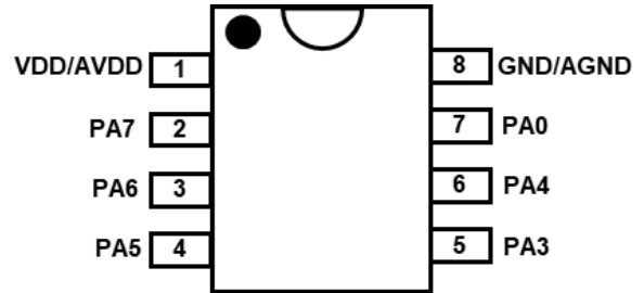
PFS123B-S08A: SOP8 (150mil)
