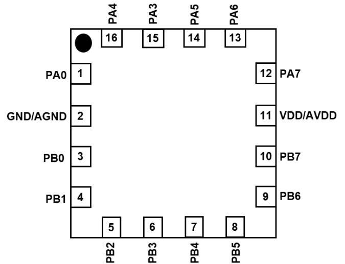
PFS123B-1J16A: QFN3*3-16P (0.5pitch)
