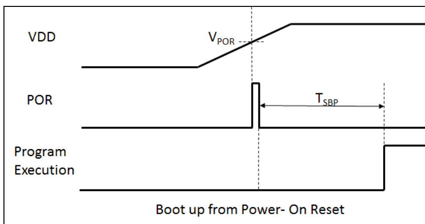
Fig.1: Power-Up Sequence
