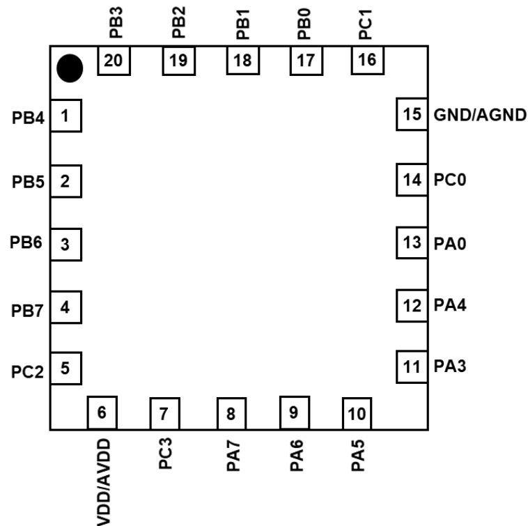
PFS123B-1J20A: QFN3*3-20P
