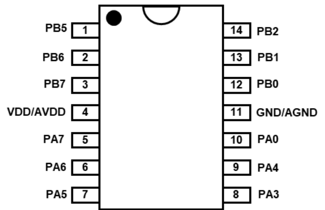
PFS123B-S14A: SOP14 (150mil)
