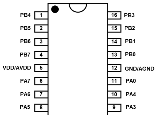
PFS123B-S16A: SOP16 (150mil)
