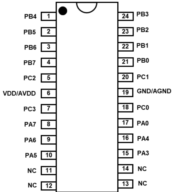
PFS123B-Y24A: SSOP24(150mil)
