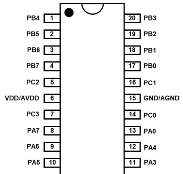
PFS123B-S20A: SOP20 (300mil)
