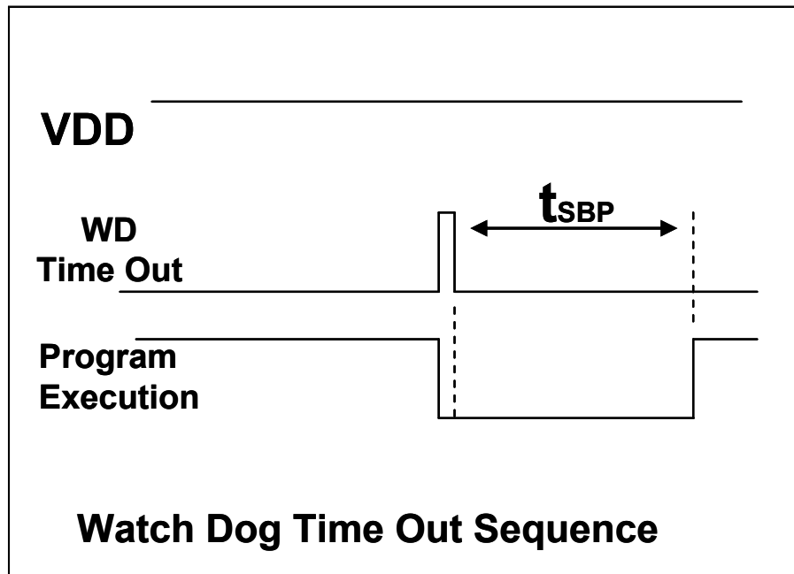
Fig.19: Sequence of Watch Dog Time Out
