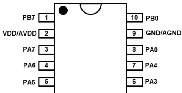
PFS123B-M10A: MSOP10 (118mil)
