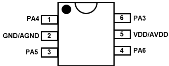
PFS123B-U06A: SOT23-6 (60mil)
